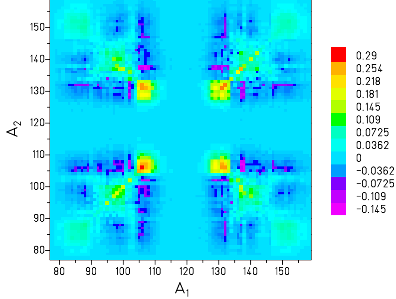
Figure 19: Covariance matrix of the fission-fragment mass yields after prompt-neutron emission from the thermal-neutron-induced fission of ^{239}\text{Pu} .
