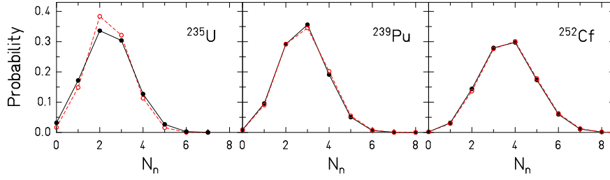
Figure 88: Measured distribution of prompt-neutron multiplicities in ^{235}\text{U}(\text{n}_{th},\text{f}) , ^{239}\text{Pu}(\text{n}_{th},\text{f}) and ^{252}\text{Cf}(\text{sf}) (data from refs. [173, 174]) (black full points) in comparison with the result of the GEF code (red open points).
