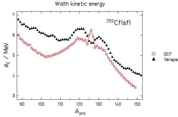
Figure 131: Width of total-kinetic-energy distribution for ^{252}\text{Cf}(sf) [232].
