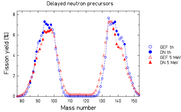
Figure 138: Mass-yield distribution for ^{235}\text{U}(\text{n},\text{f}) at thermal energy and at E_n = 5 MeV calculated with the GEF code. The full points correspond to masses with a main delayed-neutron precursor.
