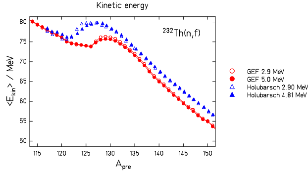
Figure 128: Mean total kinetic energy before evaporation as a function of the mass of the fragment for ^{232}\text{Th(n,f)} [231].
