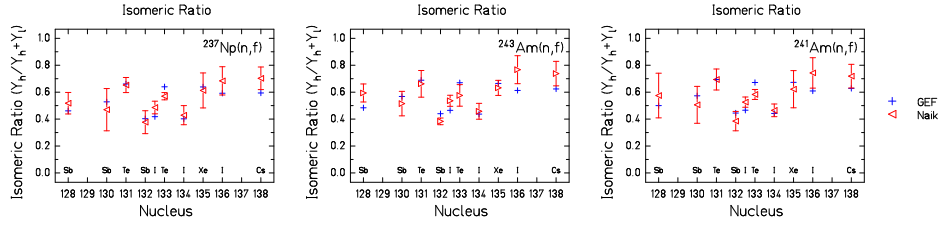
Figure 76: Isomeric ratio for odd- Z compound nuclei : ^{237}\text{Np} ( 5/2+ ) ( n,f ), ^{241}\text{Am} ( 5/2- ) ( n,f ), ^{243}\text{Am} ( 5/2+ ) ( n,f ) [163].
