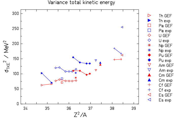
Figure 130: Variance of the TKE distribution before prompt-neutron evaporation for neutron-induced reactions, ref. [230] page 325.
