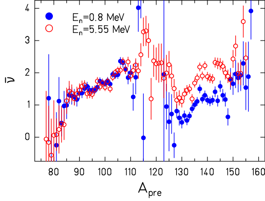
Figure 13: Prompt-neutron multiplicity as a function of the pre-neutron fragment mass for the system ^{237}\text{Np}(n,f) for E_n = 0.8 MeV and 5.55 MeV [57].
