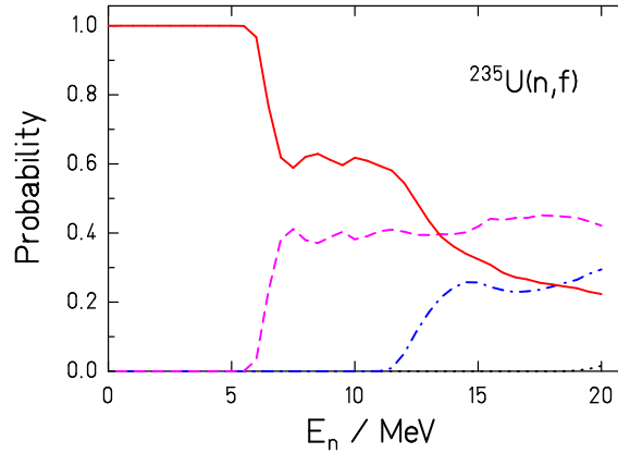
Figure 17: Relative contributions of the different fission chances to the fission events of the system ^{235}\text{U}(\text{n},\text{f}) as a function of the energy of the incident neutron. Full line: first-chance fission, dashed line: second-chance fission, dot-dashed line: third-chance fission.
