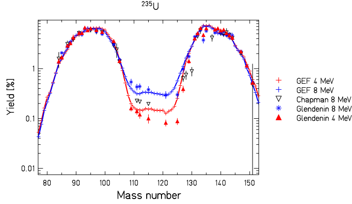
Figure 71: Fission-yield distribution for ^{235}\text{U}(n,f) for E_n = 4 MeV and E_n = 8 MeV [152, 159].
