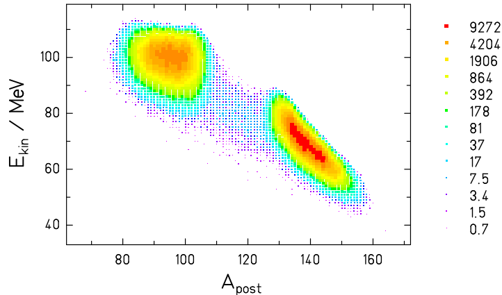
Figure 14: Calculated 2-dimensional A - E_{kin} distribution for the system ^{235}\text{U}(\text{n}_{th}, \text{f}) . The colour scale gives the number of events per channel.
