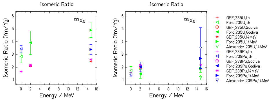
Figure 81: Isomeric ratio for ^{133}\text{Xe} and ^{135}\text{Xe} from ^{235}\text{U}(\text{n},\text{f}) and ^{239}\text{Pu}(\text{n},\text{f}) [166].
