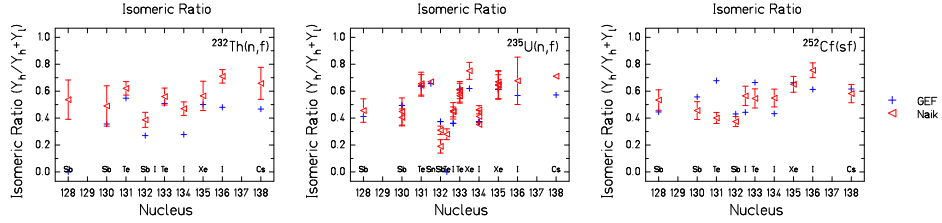
Figure 77: Isomeric ratio for even- Z compound nuclei : ^{232}\text{Th} ( 0+ ) ( n,f ), ^{235}\text{U} ( 7/2- ) ( n,f ), ^{252}\text{Cf} ( 0+ ) ( sf ) [160].
