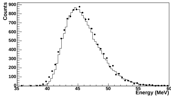
Fig. 10. Comparison between the deposited energy distribution predicted by GEANT4 (histogram) and the measured one (symbols, energy reduced by 5.5%) for 1.7 GeV/nucleon \alpha particles.
