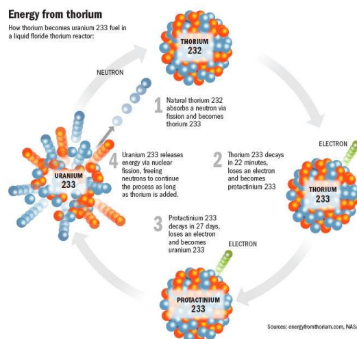
FIGURE 1.7: Cycle du thorium.
