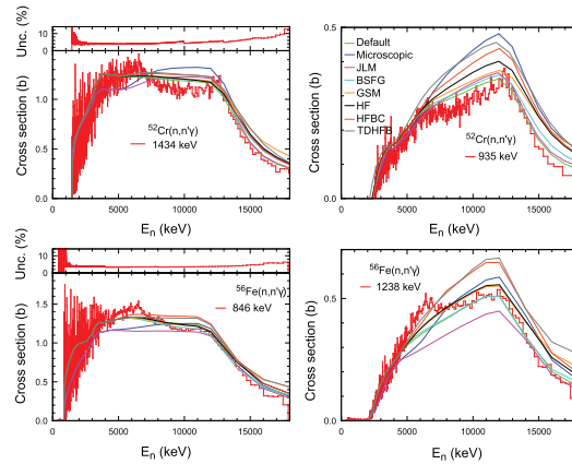
Fig. 23. (Color online) Gamma production cross sections for the transition from the first excited level to the ground state (left column) and from the second level to the 1st excited level (right column) for ^{52}\text{Cr} (corrected data) and ^{56}\text{Fe} . The data in red are compared with various model calculations performed with TALYS-1.6 (see text for details).
