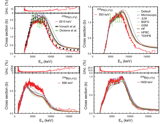
Fig. 24. (Color online) Gamma production cross sections for the transition from the first excited level to the ground state (left column) and from the second level to the 1st excited level or ground state ( ^{209}\text{Bi} ) for ^{208}\text{Pb} (corrected data) and ^{209}\text{Bi} (corrected data). The data in red are compared with various model calculations performed with TALYS-1.6 (see text for details).
