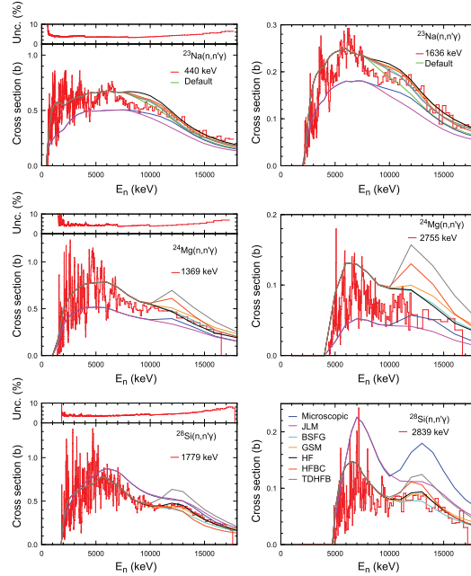
Fig. 22. (Color online) Gamma production cross sections for the transition from the first excited level to the ground state (left column) and from the second level to the 1st excited level (right column) for ^{23}\text{Na} , ^{24}\text{Mg} , and ^{28}\text{Si} . The data in red are compared with various model calculations performed with TALYS-1.6 (see text for details).
