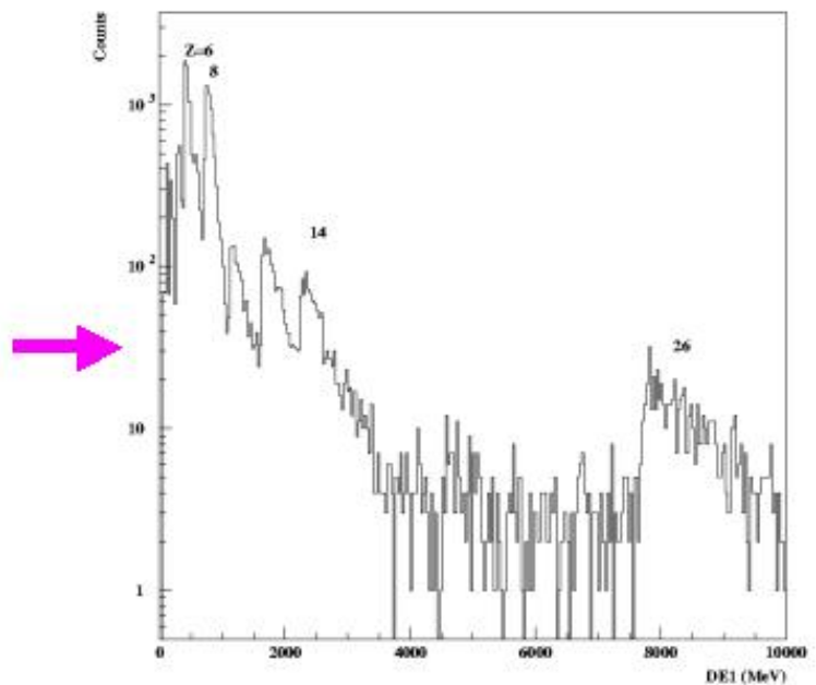
deposited-energy distributions
